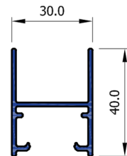
40mm Recessed Finishing Profile DW232
