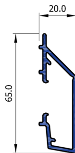
20mm Horizontal Finishing Profile DW233
