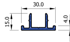
4mm Single Rail Profile DW261
