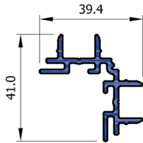
Corner Profile 90° DW250N
