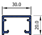
20mm Finishing Profile DW230
