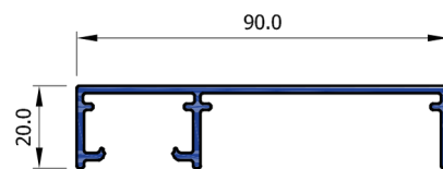
90mm Wide Finishing Profile DW240
