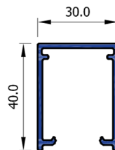
40mm Finishing Profile DW231
